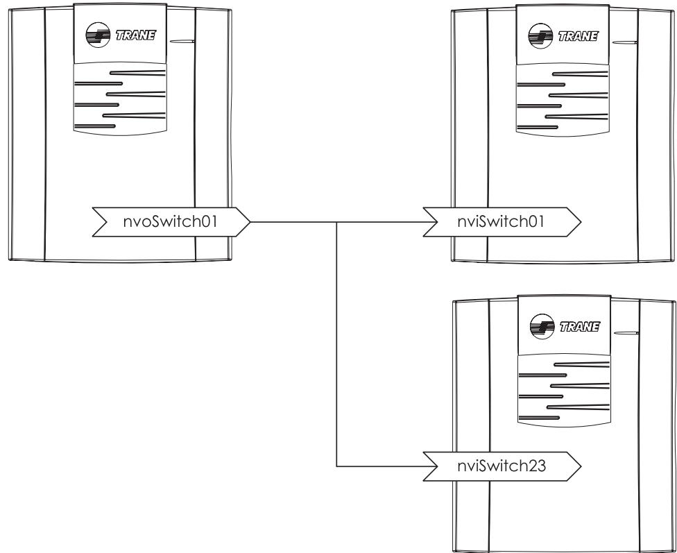
Figure 76. Group binding
